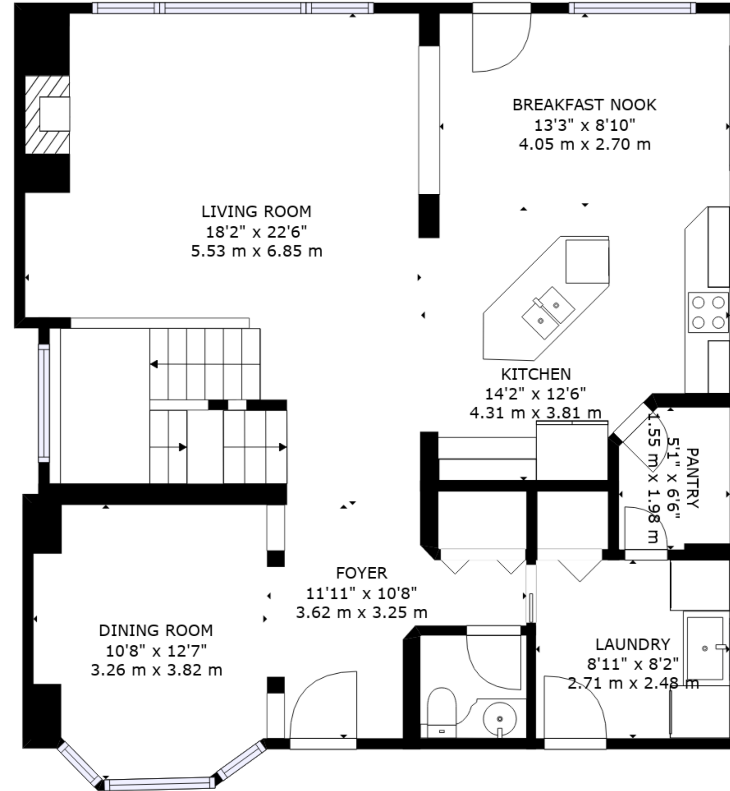
FLOOR 2
